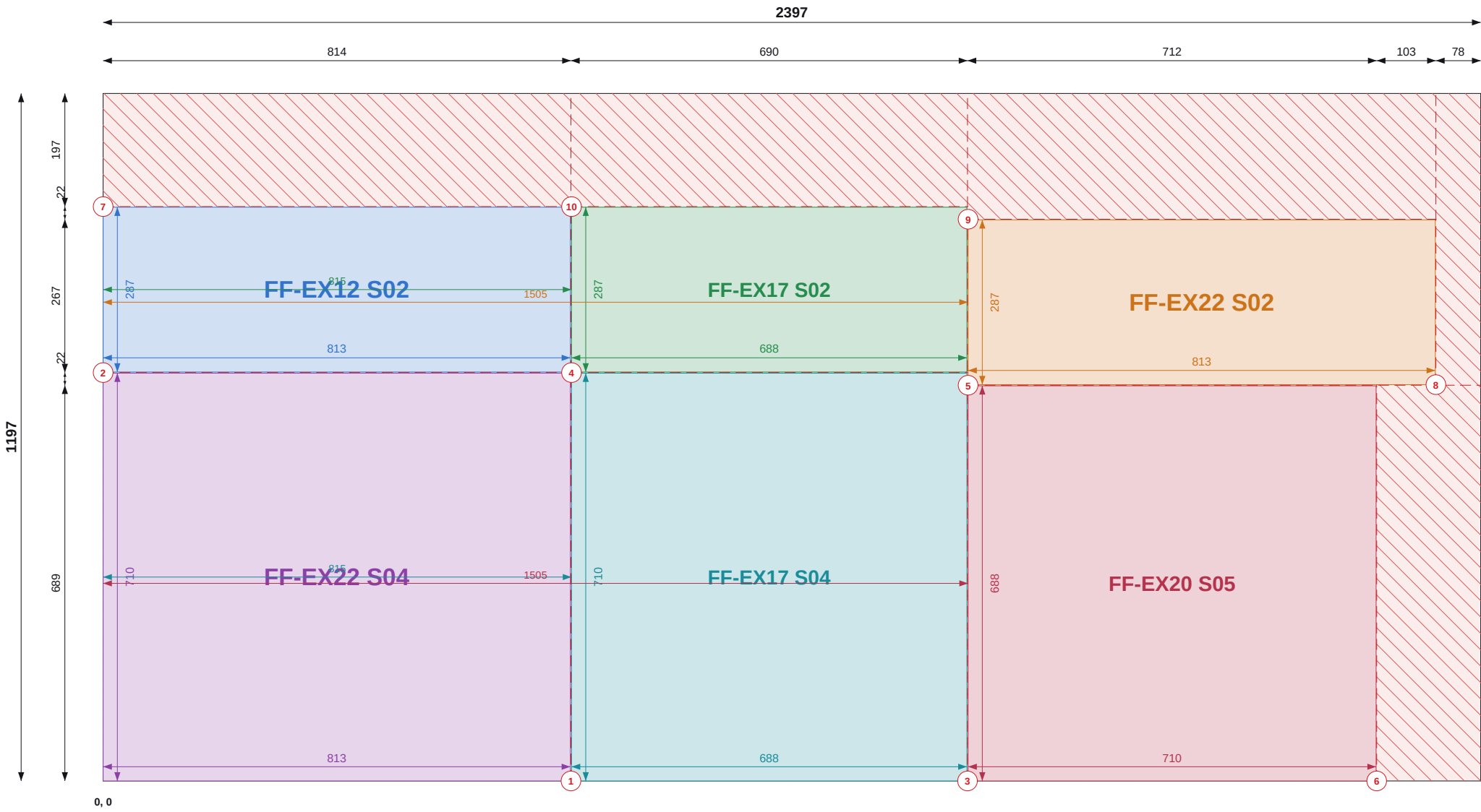
Top / left chains = saw cut positions (to cut centres). Coloured = part size and position.
